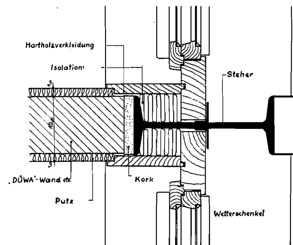
Fig. 9: Partition wall connection lining and support lining
